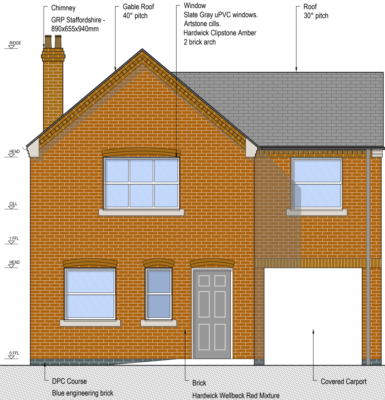
A Front Elevation
