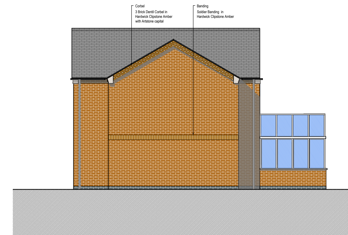
B Side 1 Elevation
