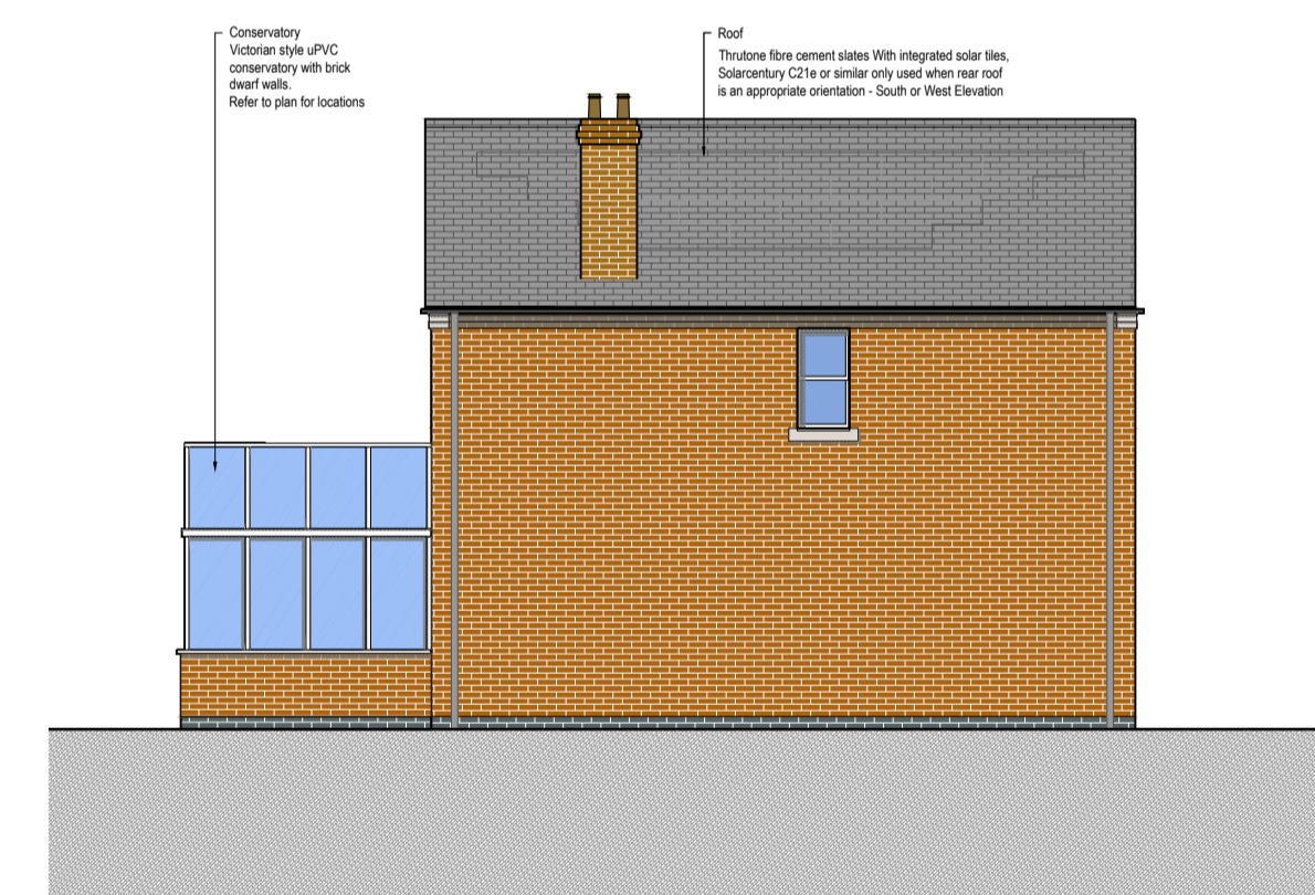
D Side 2 Elevation
